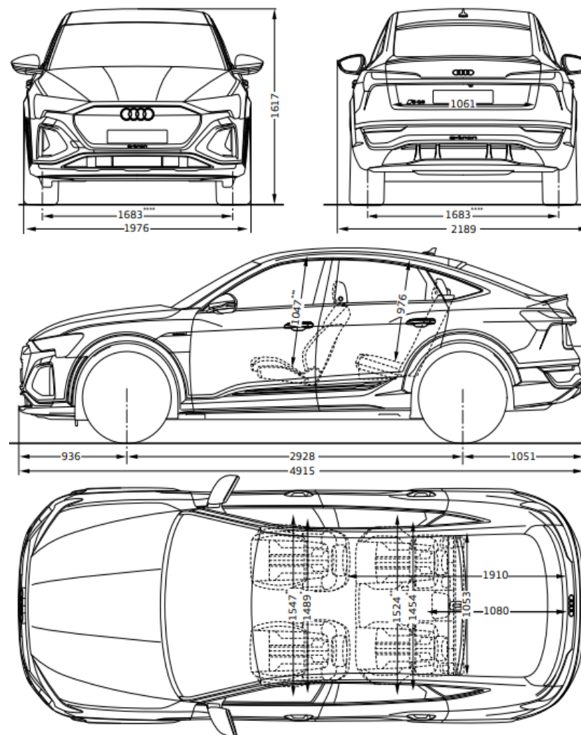
Audi SQ8 Sportback e-tron
