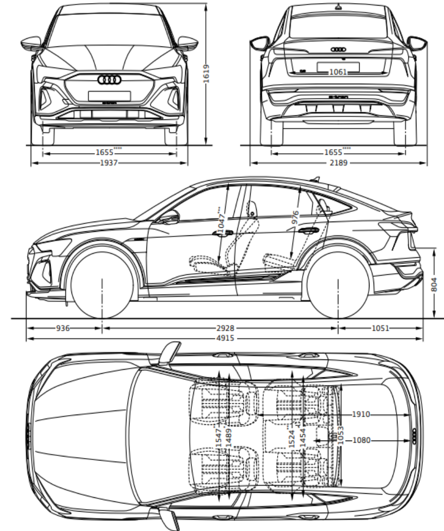
Audi Q8 Sportback e-tron
